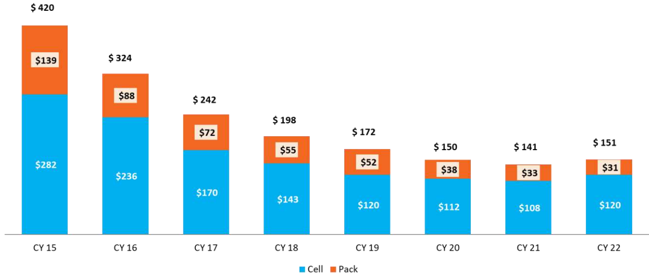
Chart 5.36: Average price of lithium-ion battery pack and cell price split, value in USD/kWh, USA, CY15-CY22
